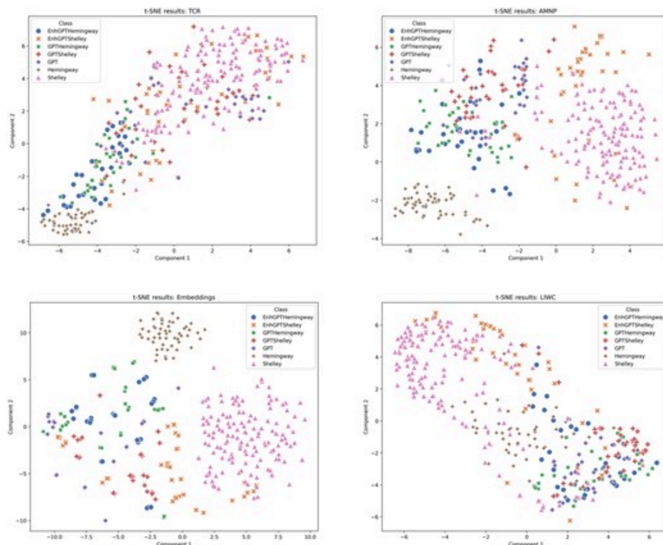
Figure 3 t-SNE plots for each feature group.
